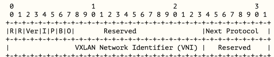
Figure 2: VXLAN-GPE Header
