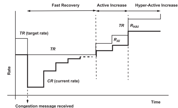
Figure 30-3—QCN RP operation
