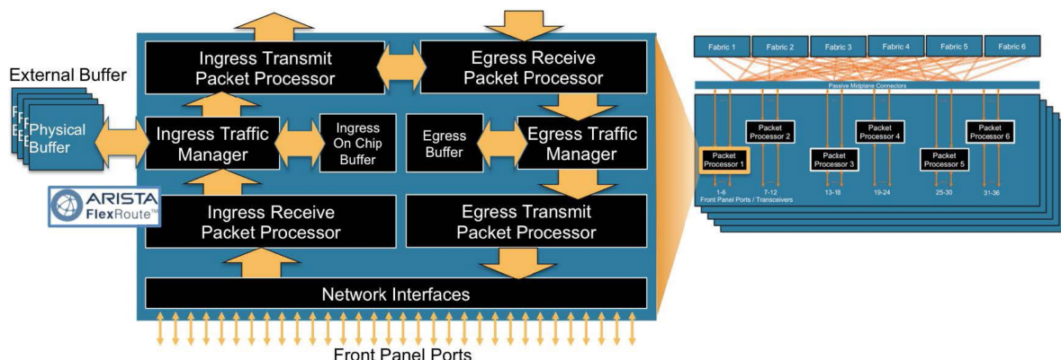
Arista 7500R Universal Spine Platform Packet Forwarding Pipeline
