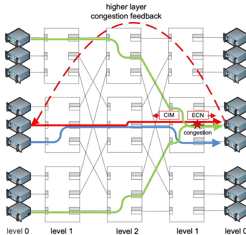
Figure 49-1—Congestion Isolation example operation
