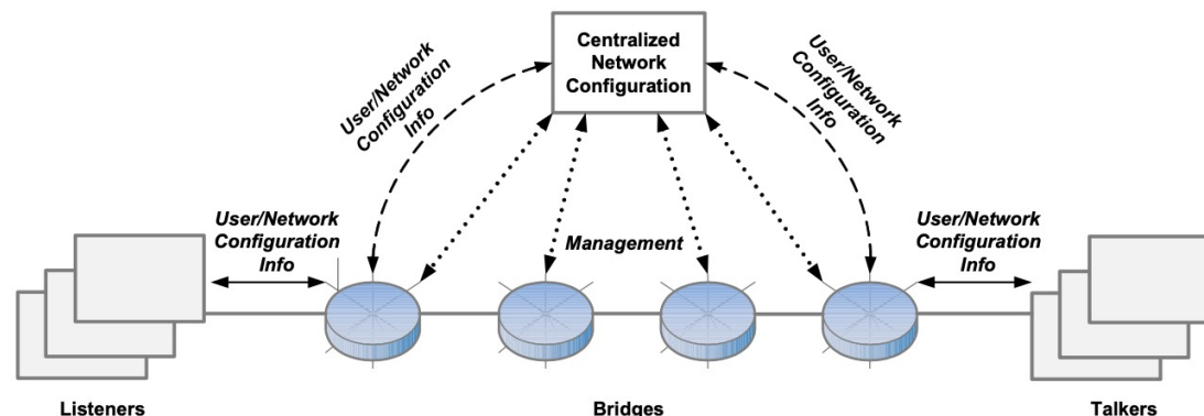
Figure 46-2—Centralized network/distributed user model
