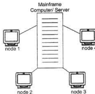
Centralised Computing
