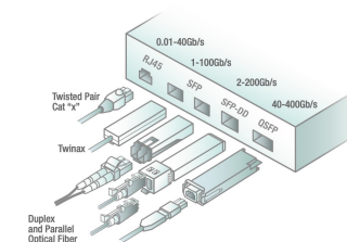
1-4 Lane Interfaces
