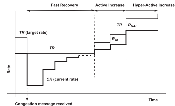
Figure 30-3—QCN RP operation
