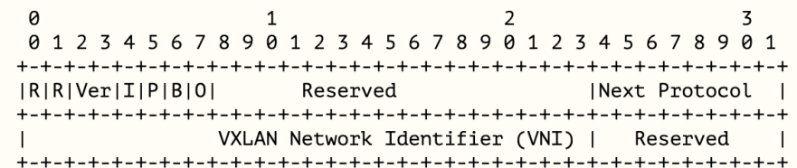
Figure 2: VXLAN-GPE Header
