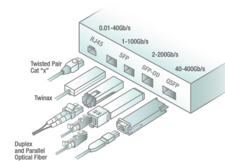
1-4 Lane Interfaces
