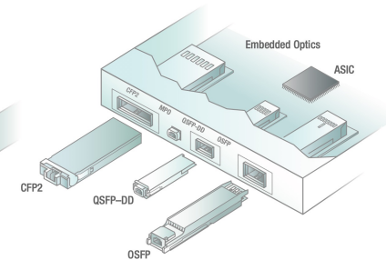
4+ Lane Interfaces
