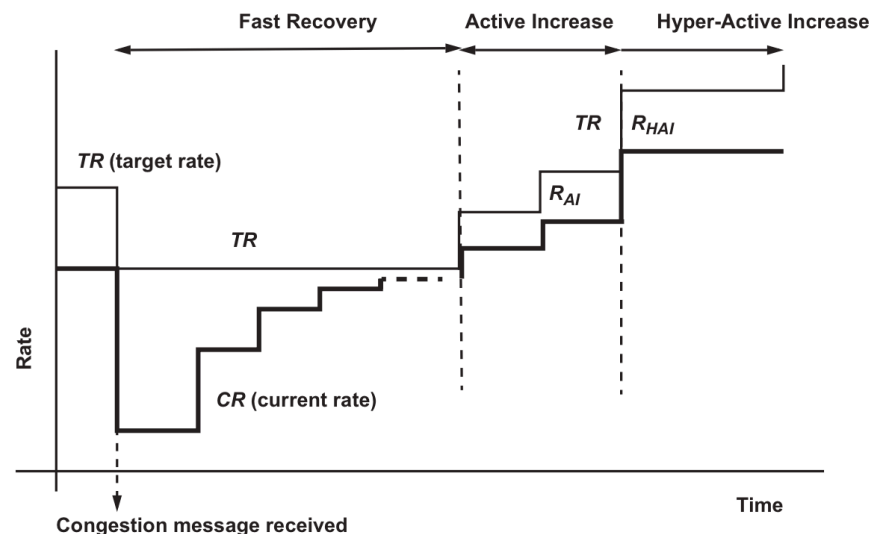
Figure 30-3—QCN RP operation
