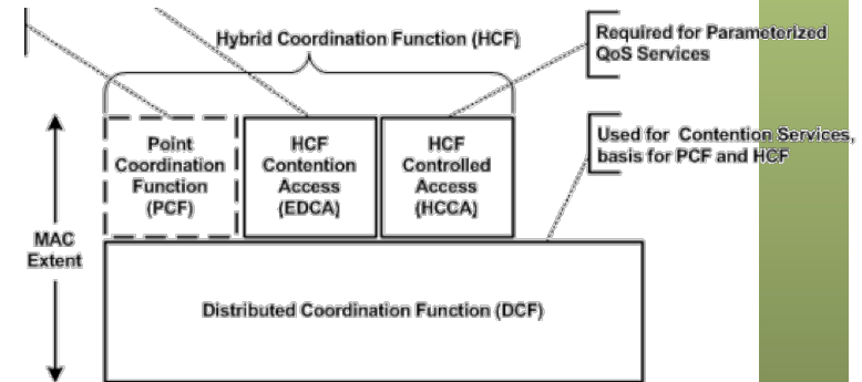
Figure 9-1—MAC architecture
