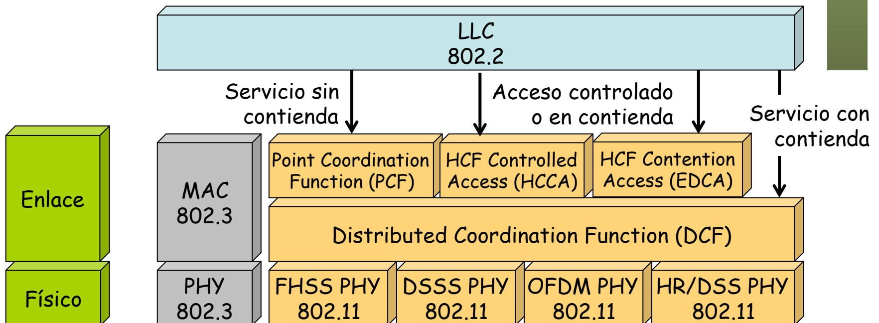
Figure 9-1—MAC architecture
