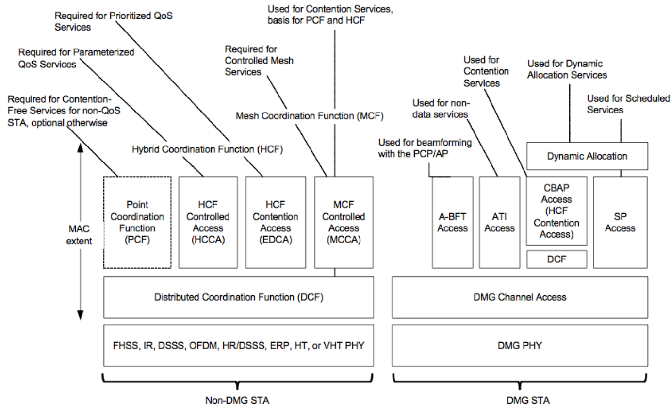
Figure 9-1—MAC architecture
