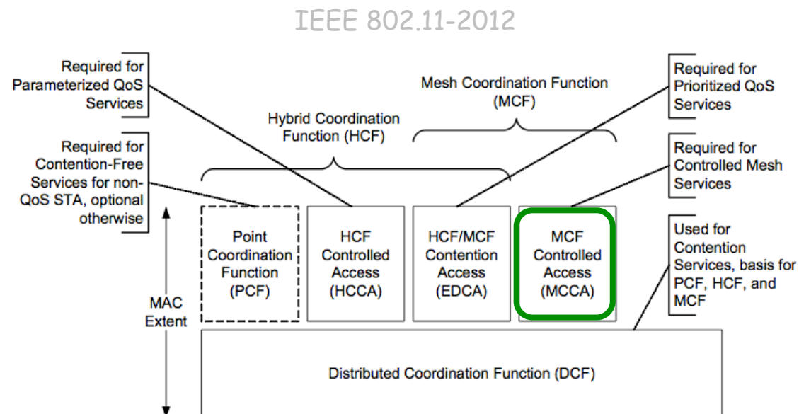
Figure 9-1—MAC architecture
