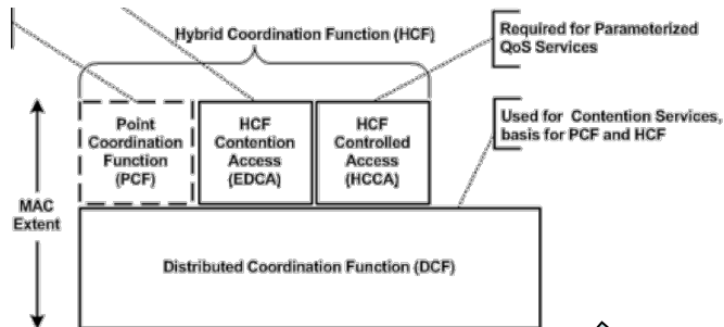
Figure 9-1—MAC architecture IEEE 802.11-2007
