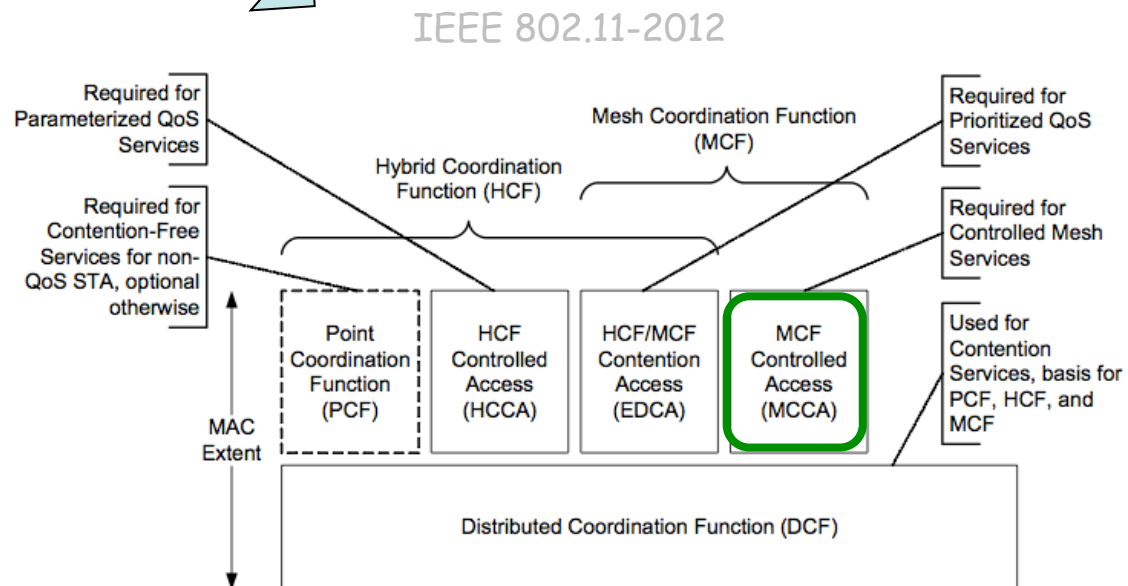
Figure 9-1—MAC architecture
