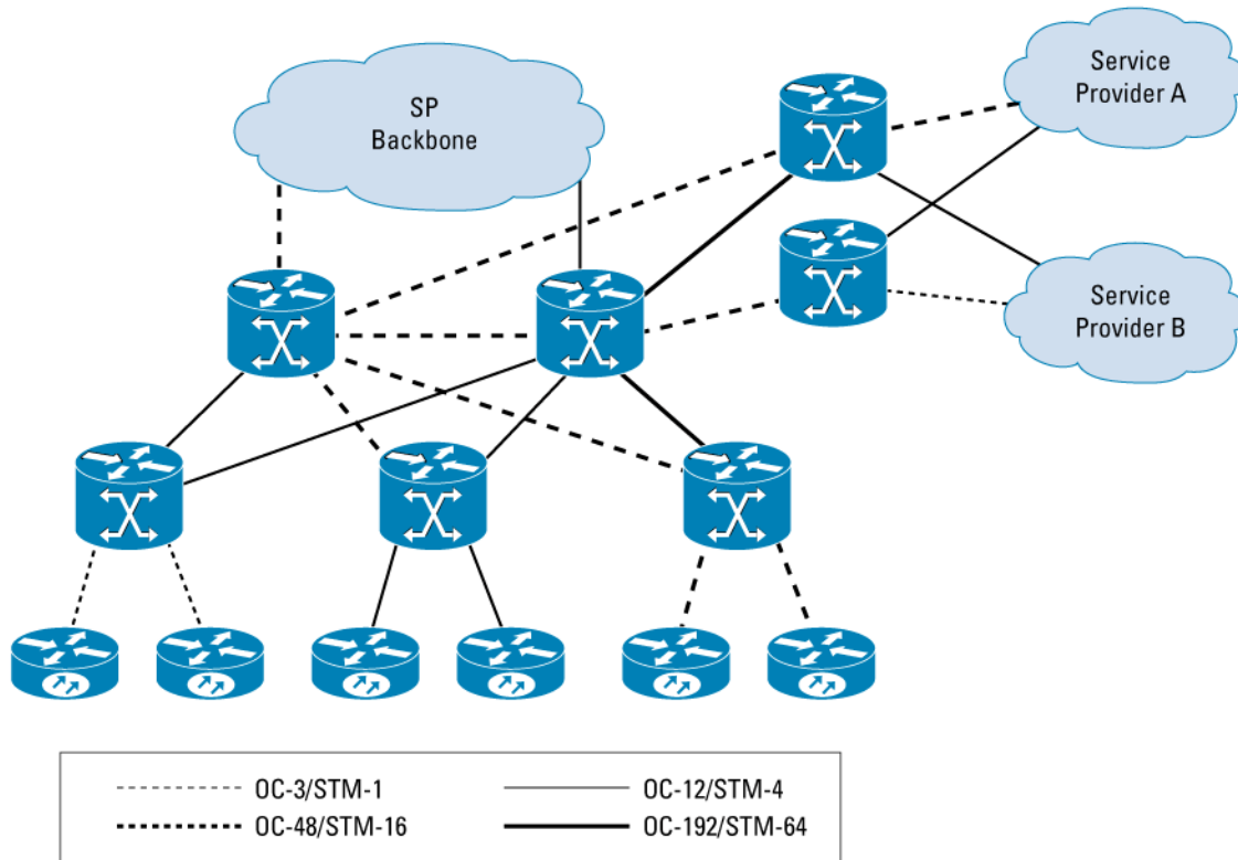
Figure 2. POS Applications
