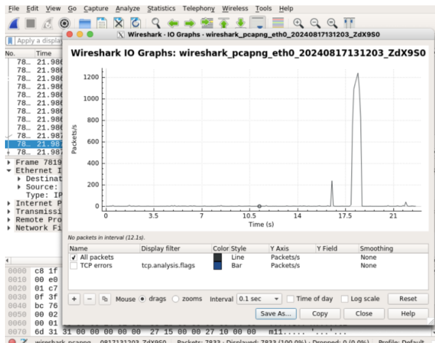
Figura 4 – I/O Graphs
