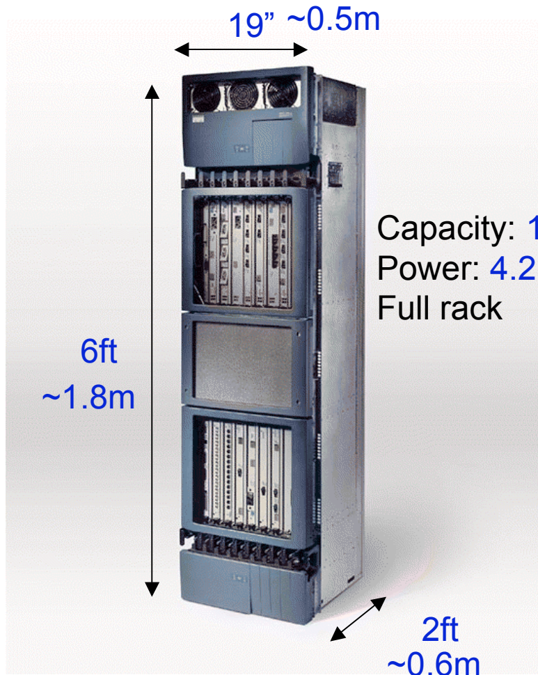
Cisco GSR 12416
