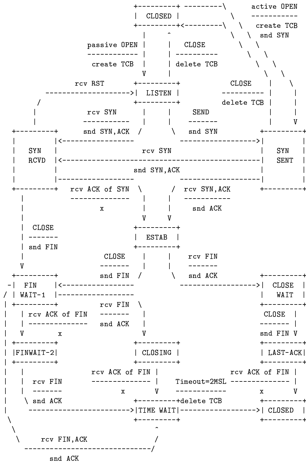
TCP Connection State Diagram
