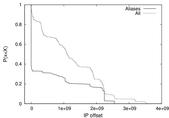
Fig. 6. IP offsets CCDF for all pairs and only aliases in Etonic infrastructure
