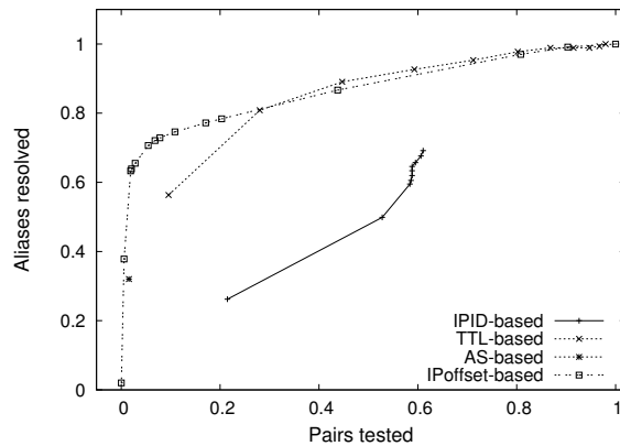
Fig. 12. Comparison of reduction methods in alias resolution
