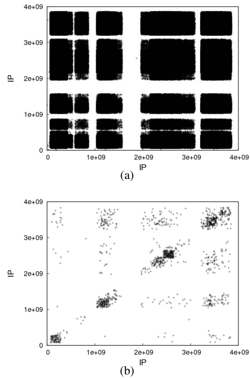
Fig. 8. IP pairs full space (a) and only alias (b) in Planetlab scenario
