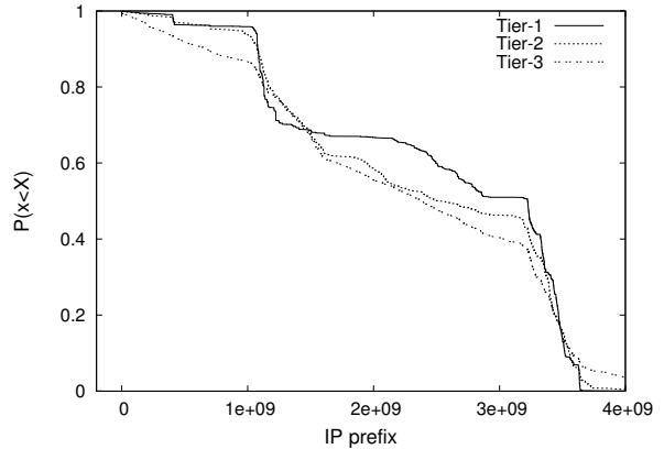
Fig. 2. CCDF of IP prefixes corresponding to Tier-1, Tier-2 and Tier-3 ASs
