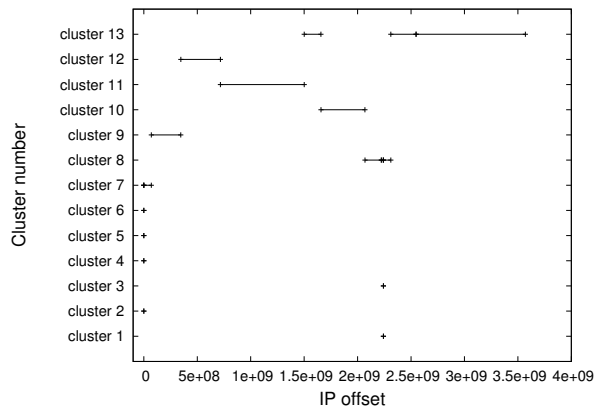
Fig. 11. IP offsets covered by each cluster
