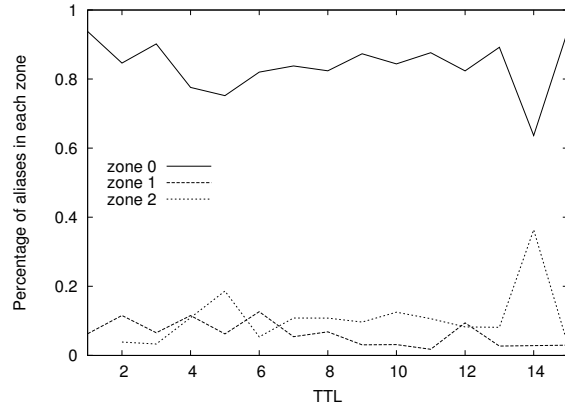
Fig. 7. Percentage of aliases found in different IP offset zone depending on the TTL distance
