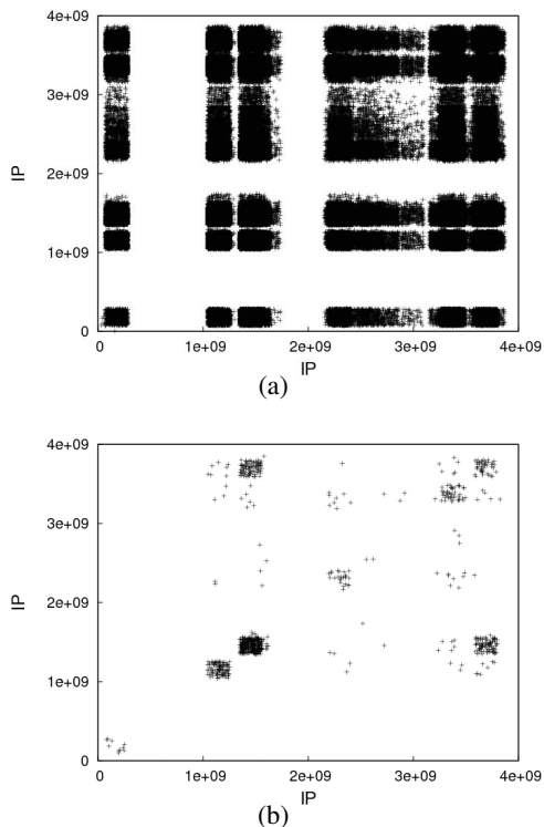
Fig. 9. IP pairs full space (a) and only alias (b) in Etomic scenario
